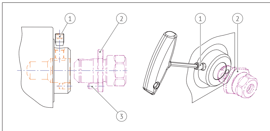
Abb. 20: easy-quick HT
